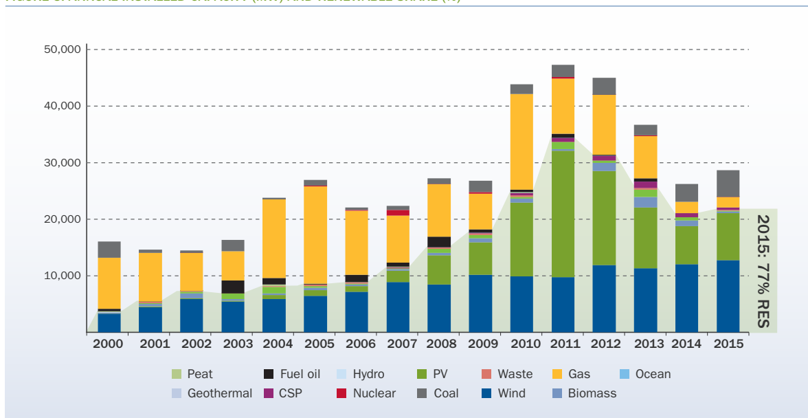
FIGURE 5: ANNUAL INSTALLED CAPACITY (MW) AND RENEWABLE SHARE (%)
