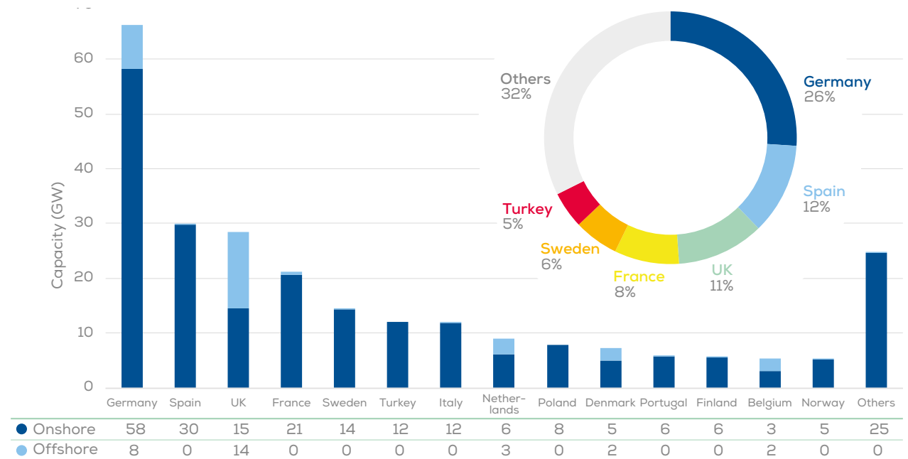
FIGURE 12. Total wind power installed capacity in by country, 2022
